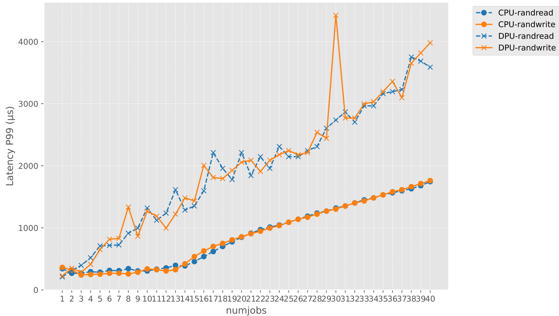
Latency P99 vs numjobs (CPU vs DPU)
